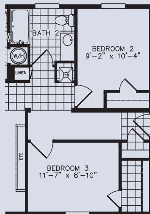
PATRIOT II OPTIONAL GABLE END ENTRY
